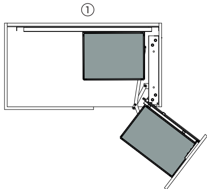
Right side magic corner
