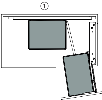
Right side magic corner
