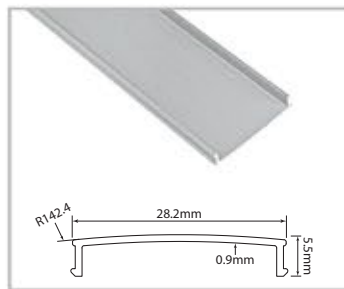
WSP-06 Sliding Top & Bottom Profile
