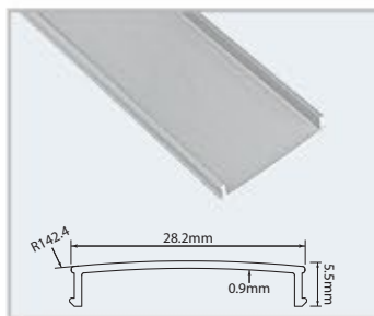
WSP-12C Bottom Cover Profile
