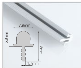
WSP-21 Sliding Bottom Profile
